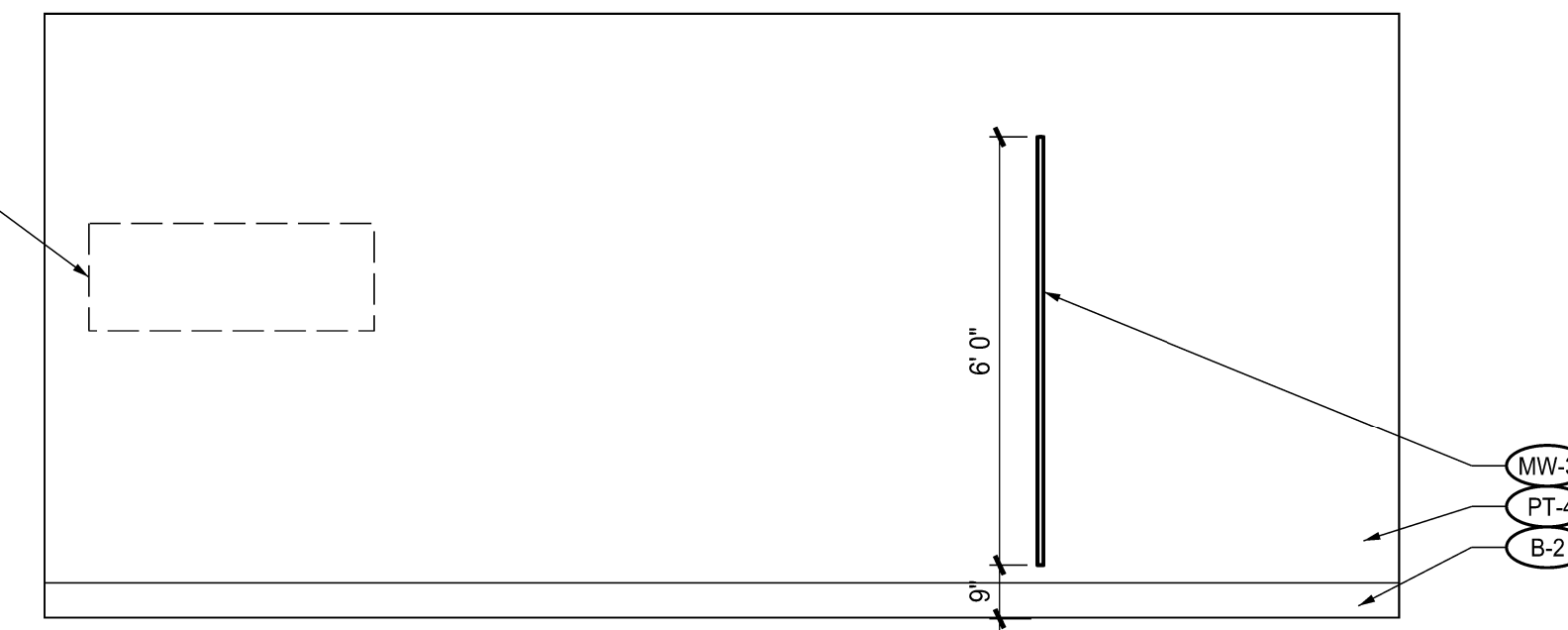
14 INTERIOR ELEVATION – RESTROOM A4.02 SCALE: 3/8" = 1'-0"
