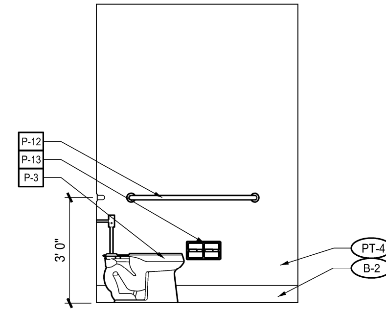
6 INTERIOR ELEVATION – RESTROOM A4.02 SCALE: 3/8" = 1'-0"
