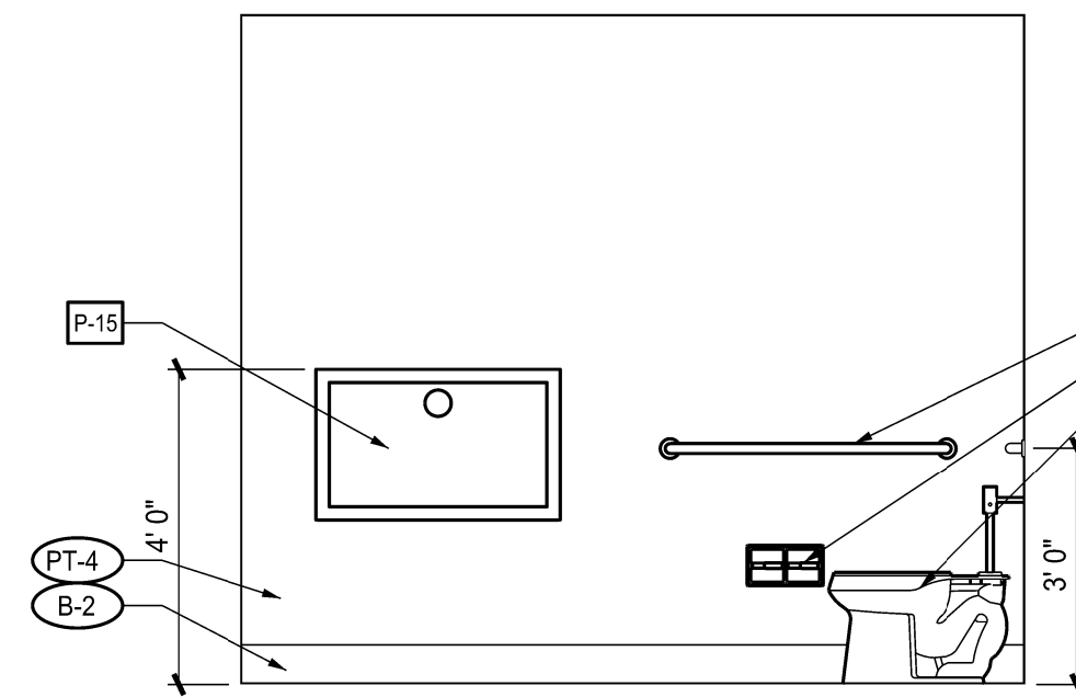
15 INTERIOR ELEVATION – RESTROOM A4.02 SCALE: 3/8" = 1'-0"
