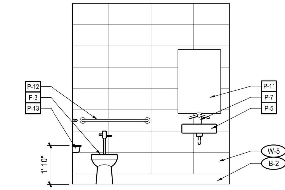
1 INTERIOR ELEVATION – RESTROOM A4.02 SCALE: 3/8" = 1'-0"
