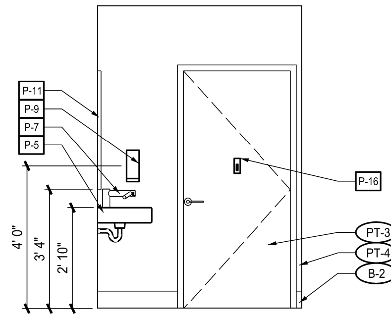
2 INTERIOR ELEVATION – RESTROOM A4.02 SCALE: 3/8" = 1'-0"
