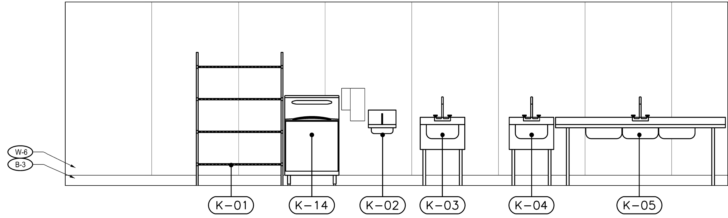
1 INTERIOR ELEVATION – KITCHEN A4.03 SCALE: 3/8" = 1'-0"
