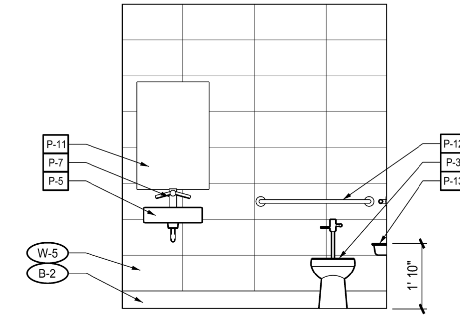
5 INTERIOR ELEVATION – RESTROOM A4.02 SCALE: 3/8" = 1'-0"
