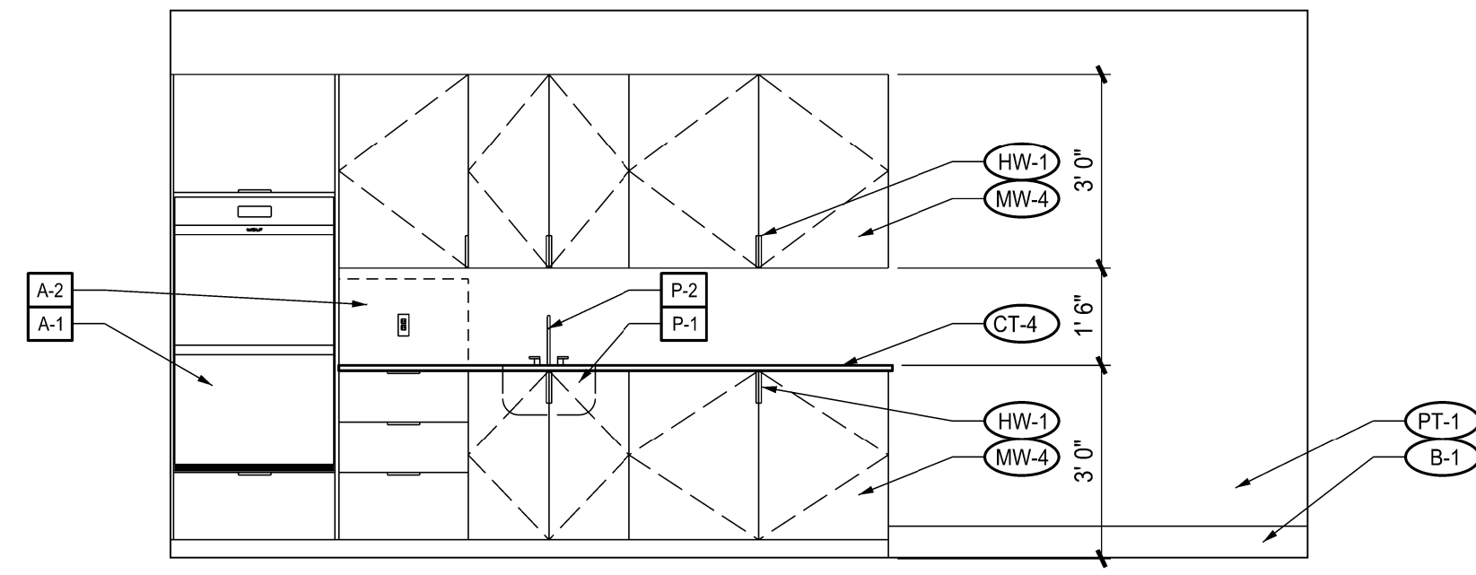
7 INTERIOR ELEVATION – BREAKROOM A4.03 SCALE: 3/8" = 1'-0"
