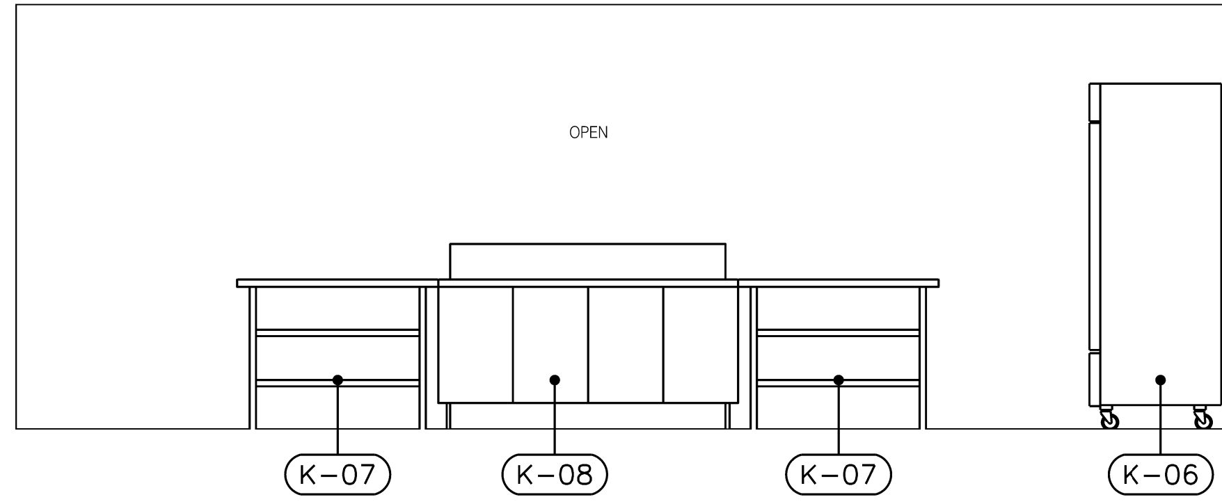
2 INTERIOR ELEVATION – KITCHEN A4.03 SCALE: 3/8" = 1'-0"
