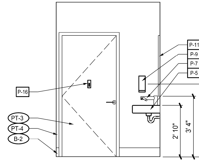
8 INTERIOR ELEVATION – RESTROOM A4.02 SCALE: 3/8" = 1'-0"
