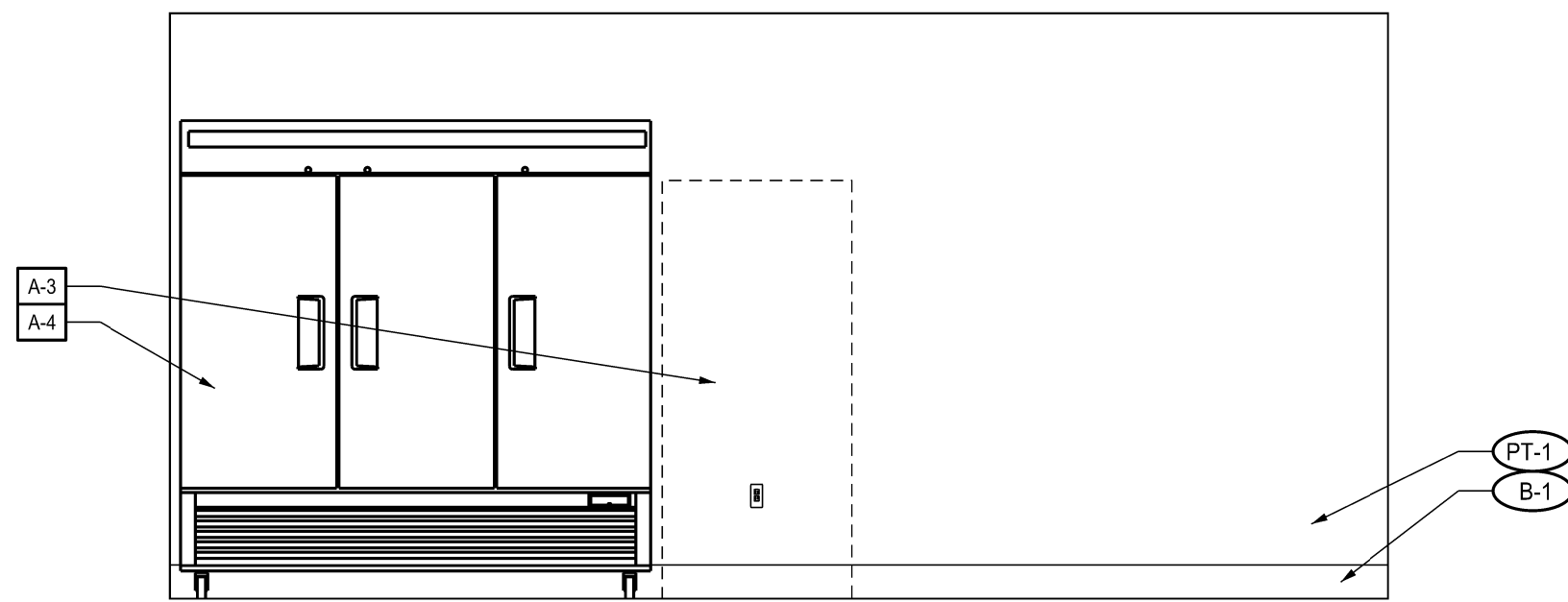
8 INTERIOR ELEVATION – BREAKROOM A4.03 SCALE: 3/8" = 1'-0"
