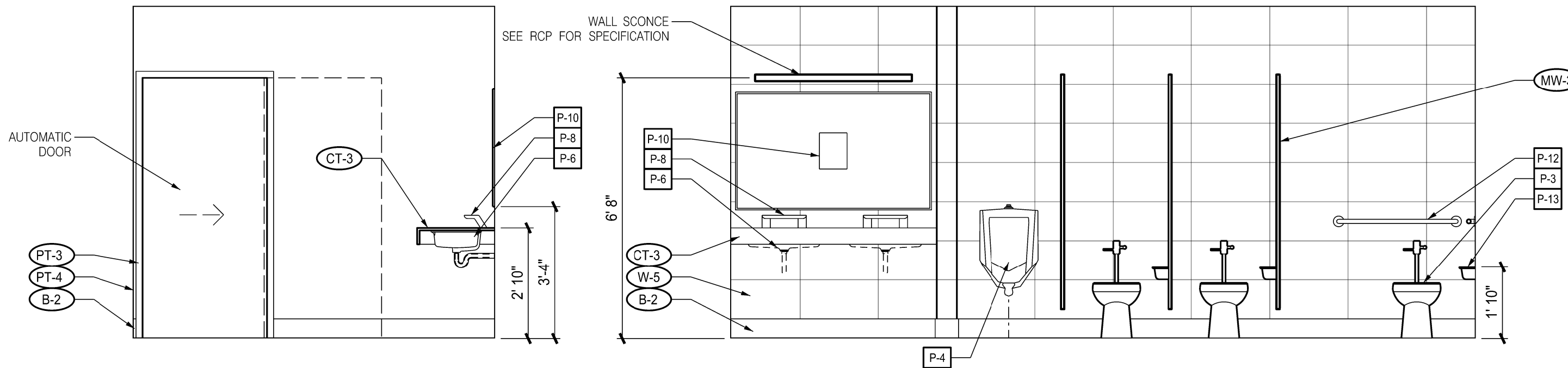
9 INTERIOR ELEVATION – RESTROOM A4.02 SCALE: 3/8" = 1'-0"
