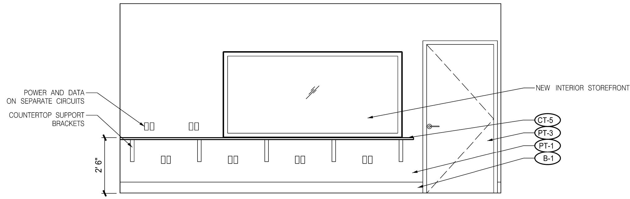
6 INTERIOR ELEVATION – PRODUCTION A4.03 SCALE: 3/8" = 1'-0"
