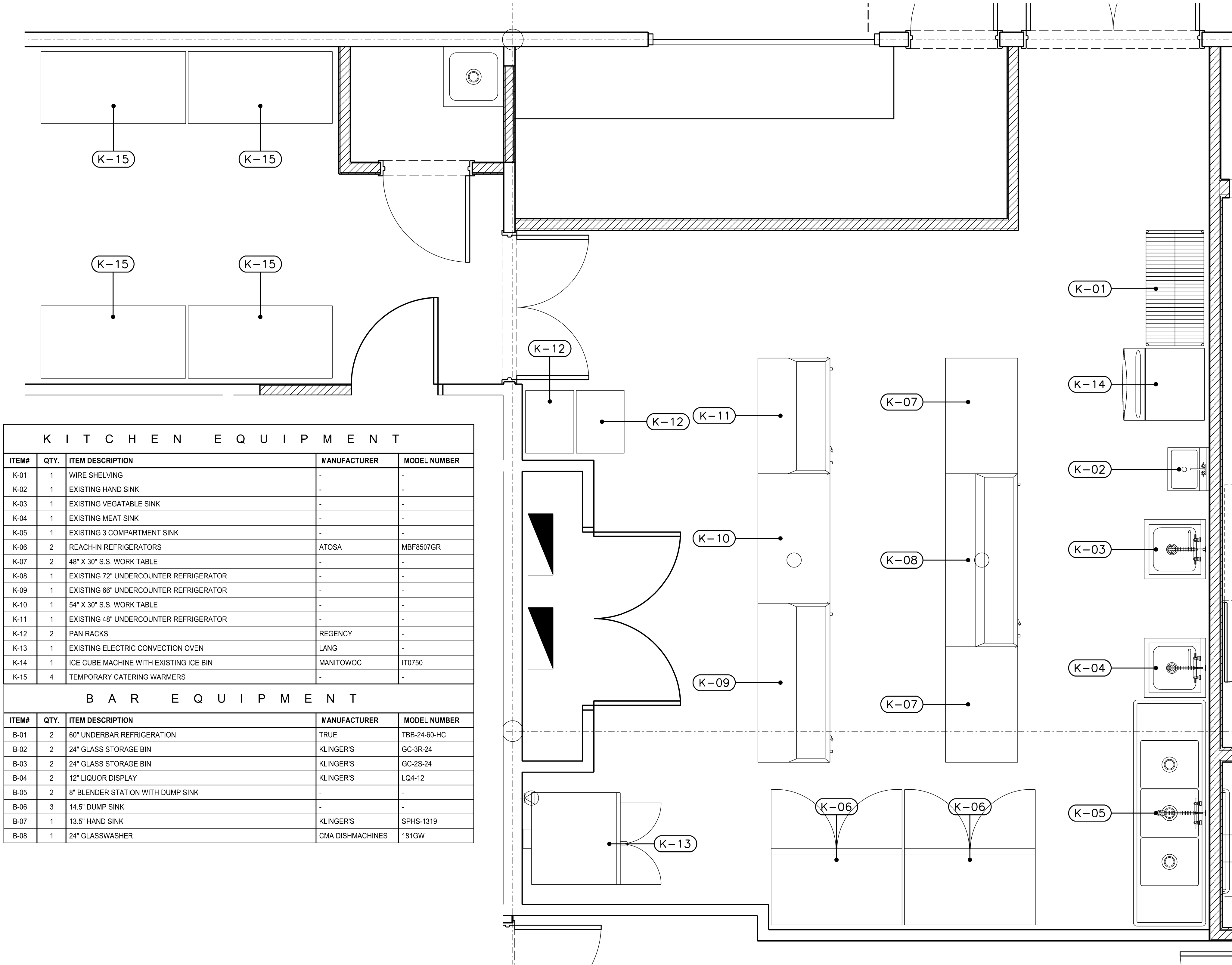
1 EQUIPMENT PLAN – CATERING KITCHEN A1.06 SCALE: 1/2" = 1'-0"
