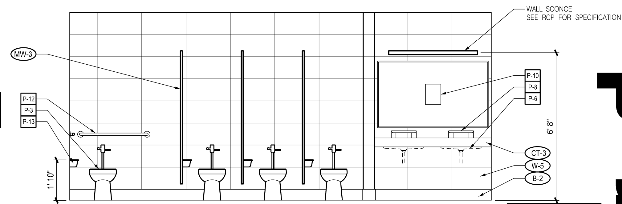
16 INTERIOR ELEVATION – RESTROOM A4.02 SCALE: 3/8" = 1'-0"
