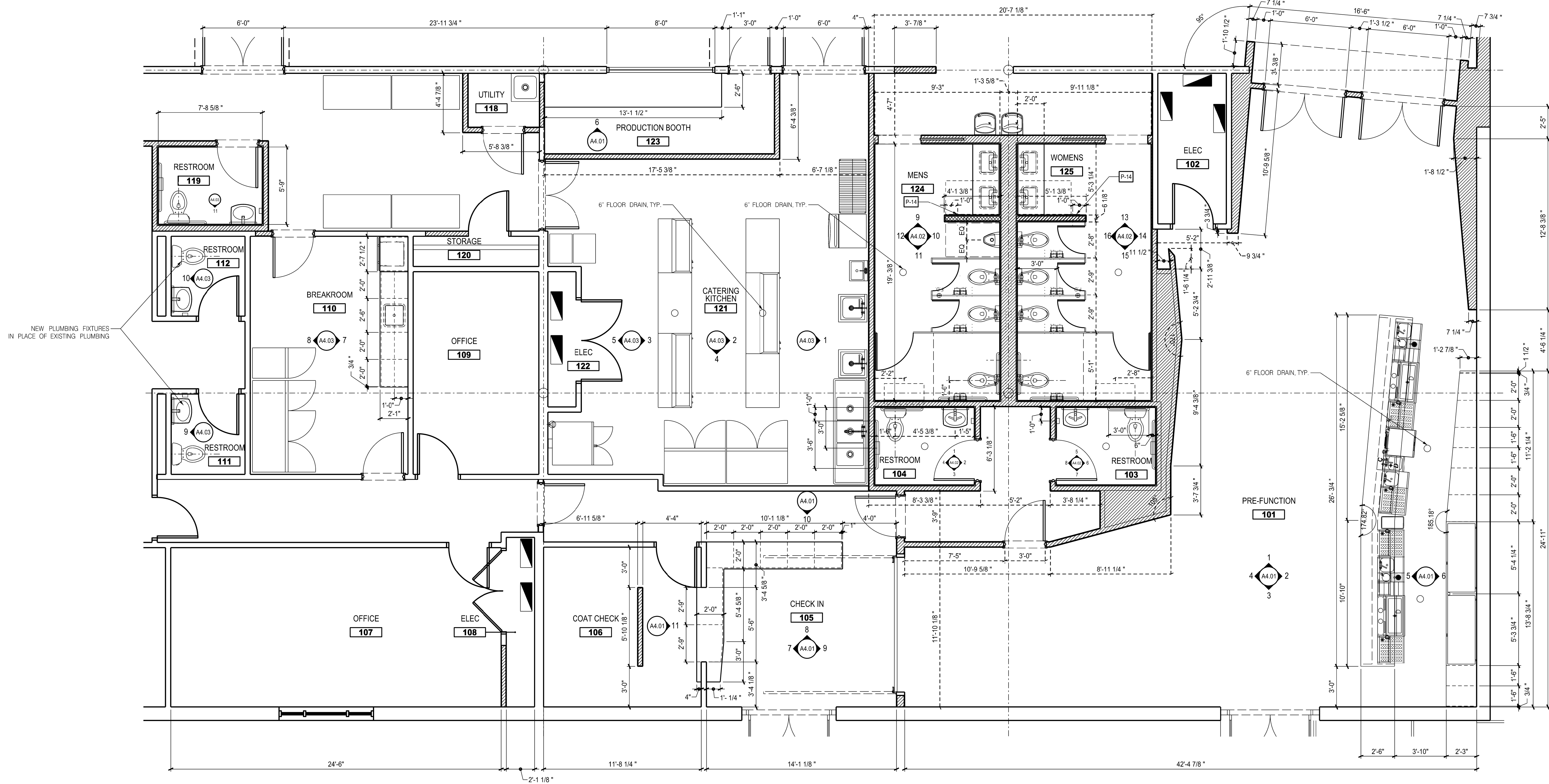
1 ENLARGED PLAN A1.03 SCALE: 1/4" = 1'-0"
