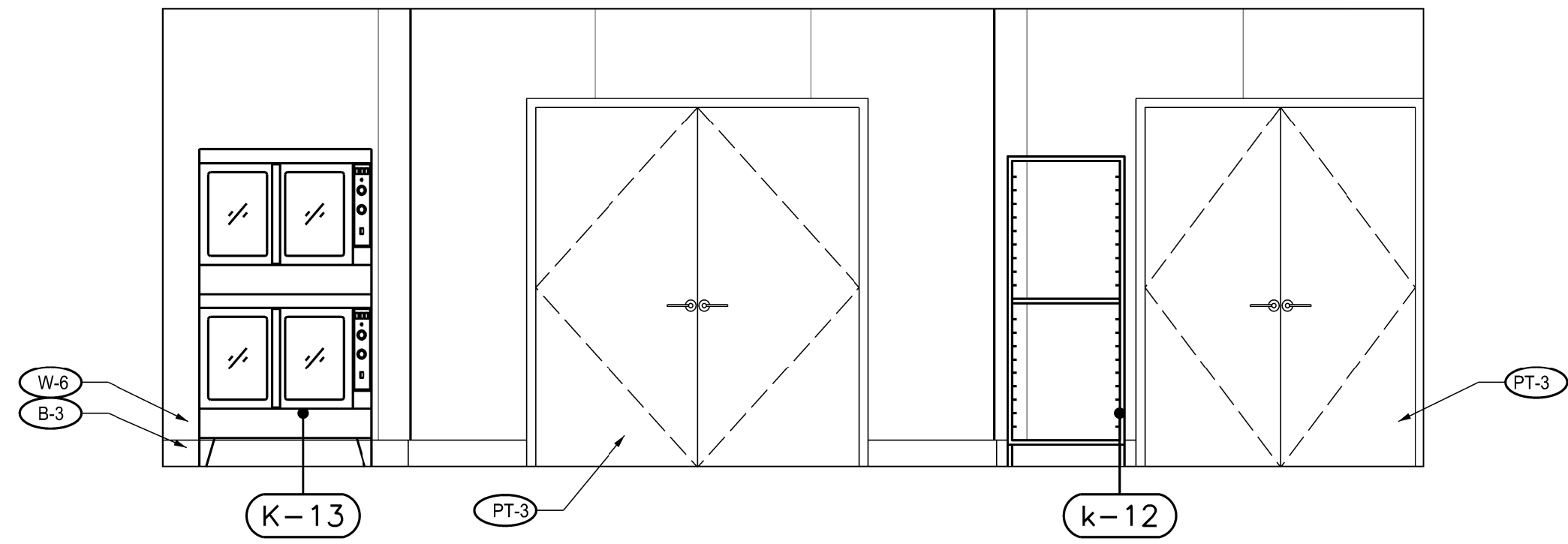
5 INTERIOR ELEVATION – KITCHEN A4.03 SCALE: 3/8" = 1'-0"
