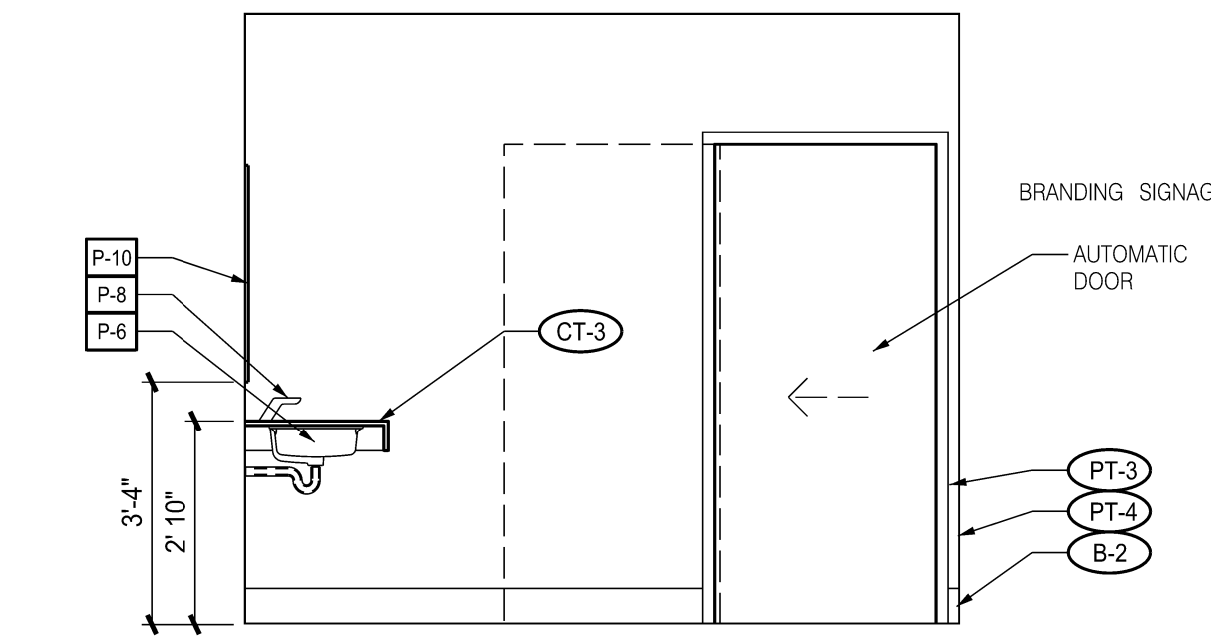
13 INTERIOR ELEVATION – RESTROOM A4.02 SCALE: 3/8" = 1'-0"
