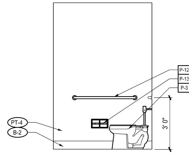
4 INTERIOR ELEVATION – RESTROOM A4.02 SCALE: 3/8" = 1'-0"
