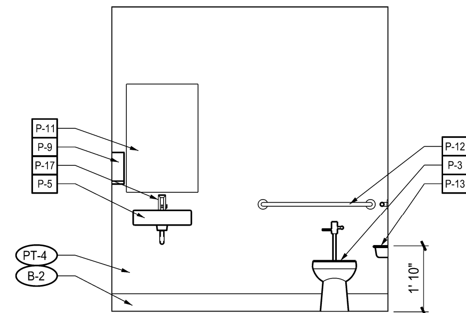
11 INTERIOR ELEVATION – RESTROOM A4.03 SCALE: 3/8" = 1'-0"
