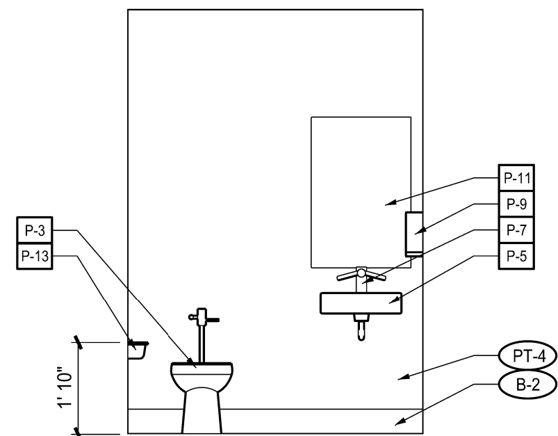
9 INTERIOR ELEVATION – RESTROOM A4.03 SCALE: 3/8" = 1'-0"
