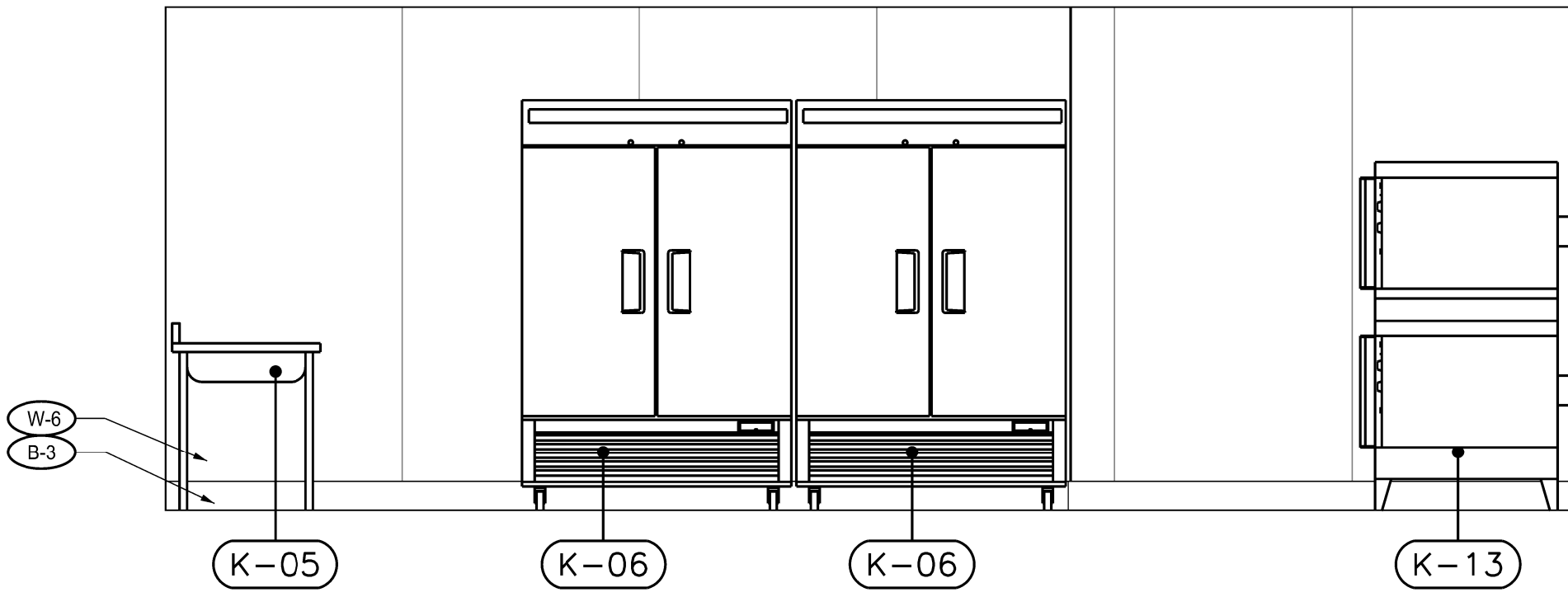
4 INTERIOR ELEVATION – KITCHEN A4.03 SCALE: 3/8" = 1'-0"
