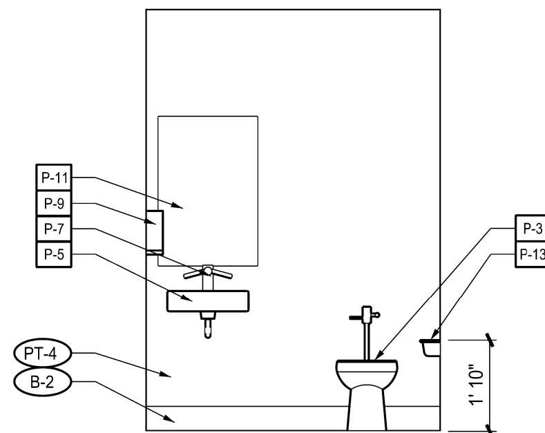
10 INTERIOR ELEVATION – RESTROOM A4.03 SCALE: 3/8" = 1'-0"
